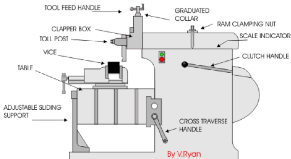
Shaping machine
