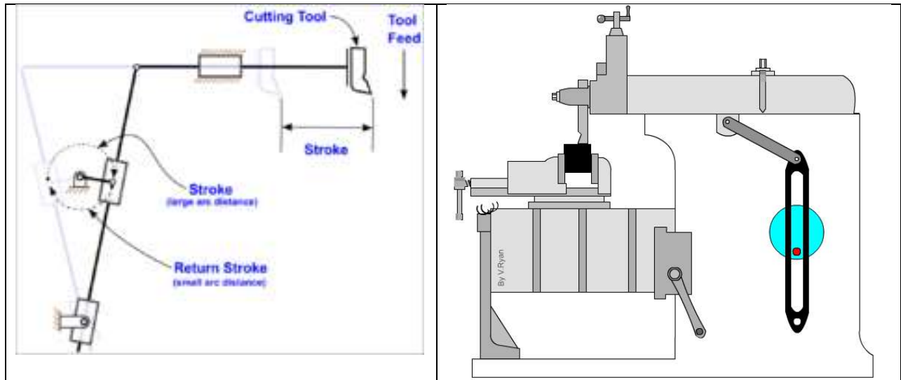
Quick return mechanism
